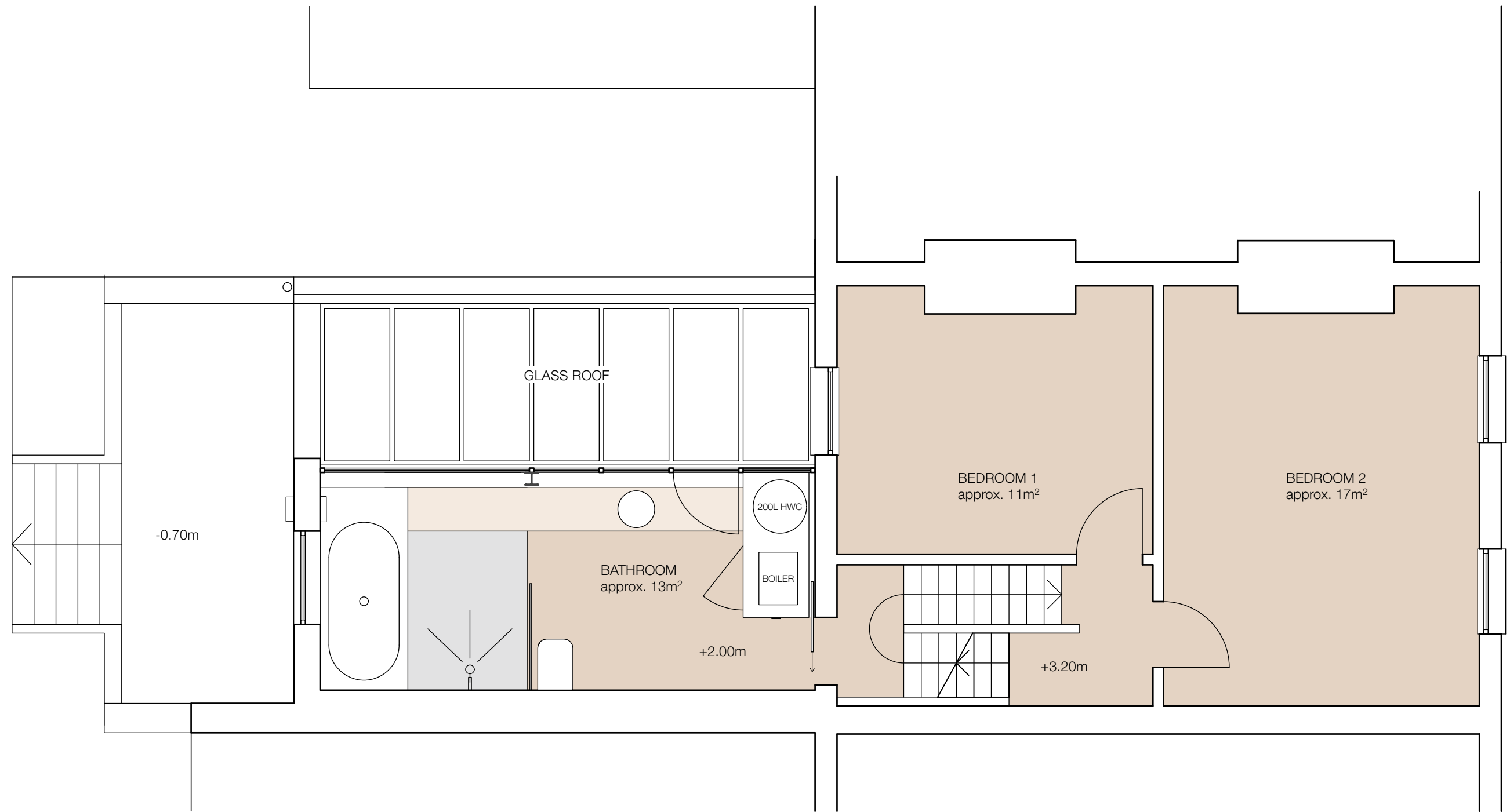
FIRST FLOOR
